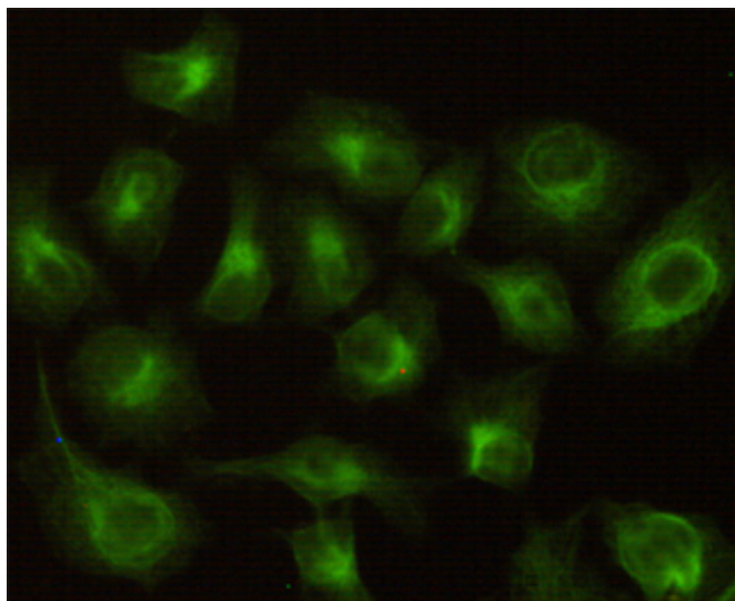
Immunocytochemistry analysis of CBR1 (2C9) in Hela using CBR1 antibody.
