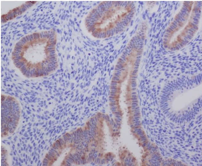
Immunohistochemistry analysis of paraffin-embedded Human uterus using AGR2 antibody. High-pressure and temperature Sodium Citrate pH 6.0 was used for antigen retrieval.
