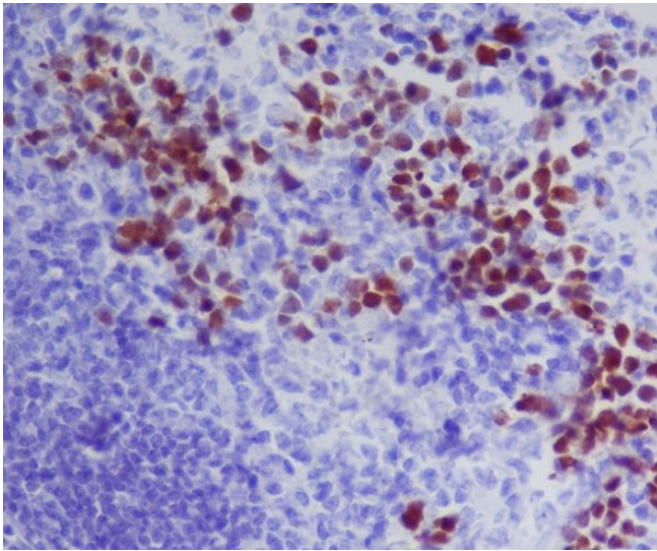
Immunohistochemistry analysis of paraffin-embedded mouse spleen using GATA1 antibody. High-pressure and temperature Sodium Citrate pH 6.0 was used for antigen retrieval.
